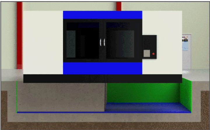
Machine tool foundation
