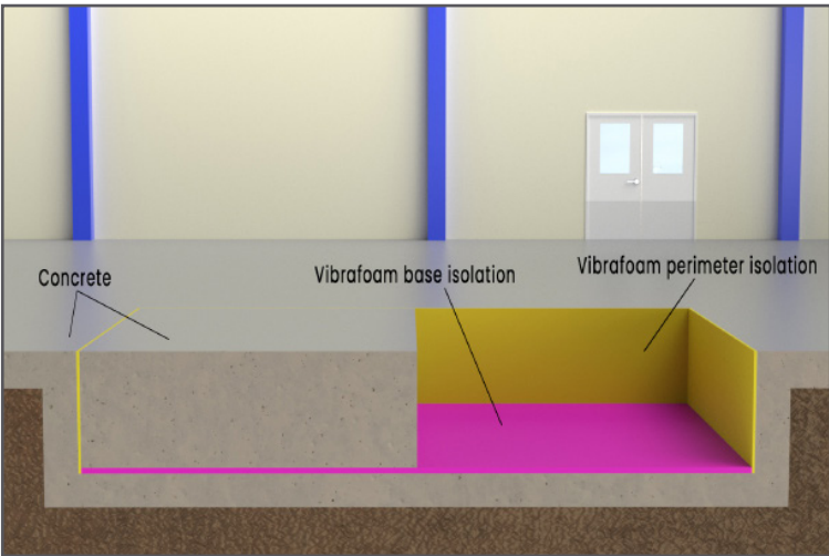
Machine Foundation
