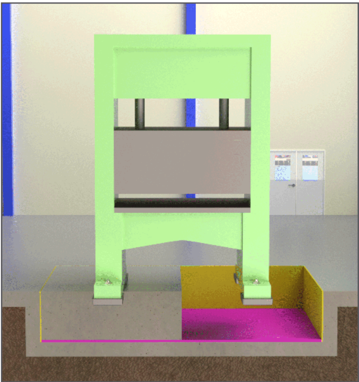
Stamping press foundation
