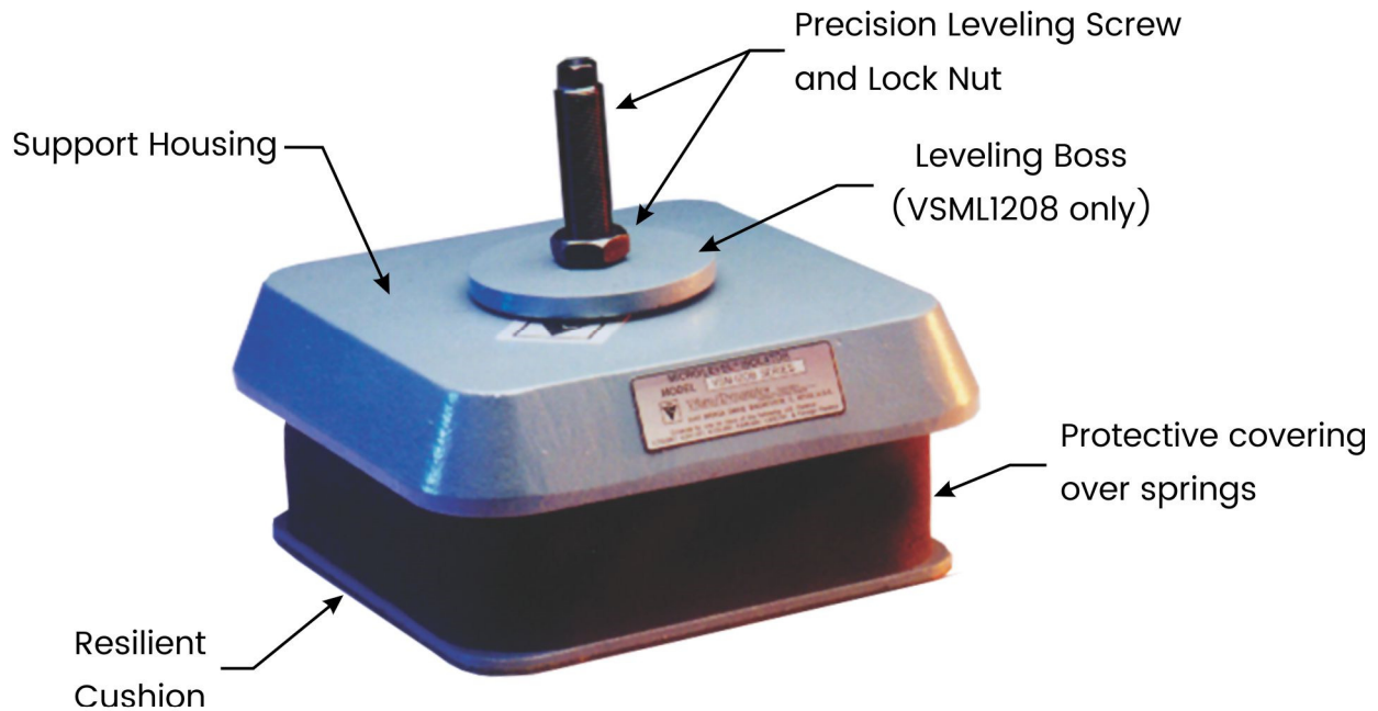
VSML1208 Hy/Speed® Isolator
